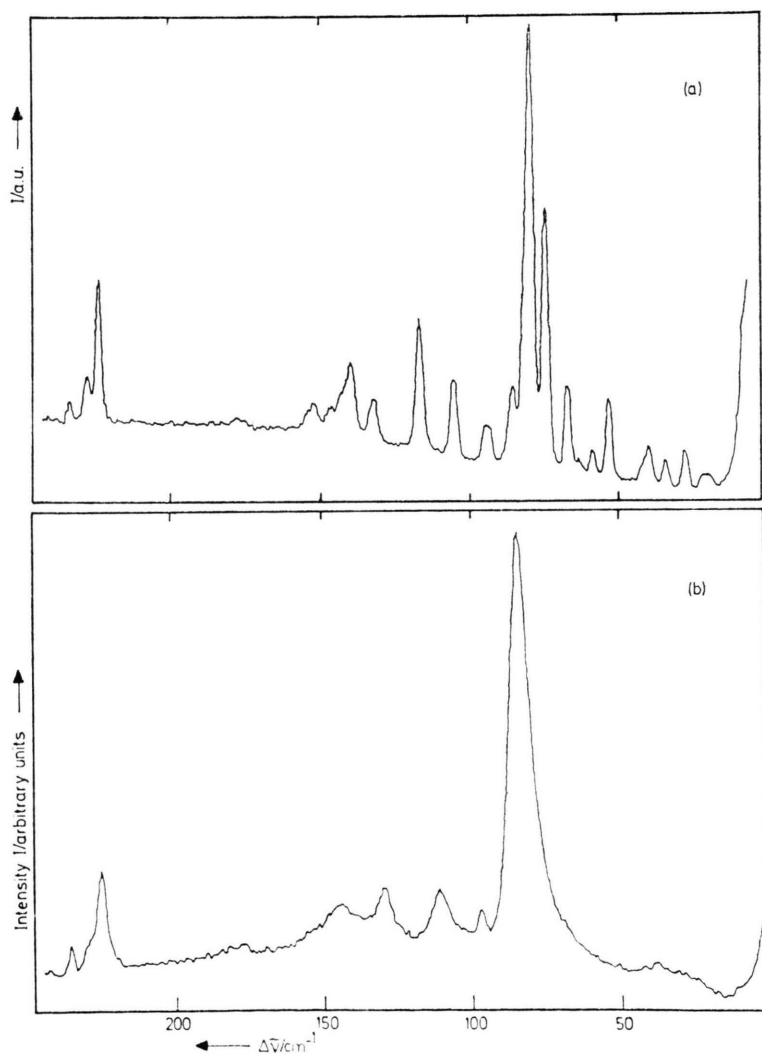
Fig. 1. Low frequency Raman spectra of Phen-TCNB (a) and Anth 0.5 Phen 0.5 TCNB (b). Excitation wavelength: 647.1 nm. Resolution: 2 \text{cm}^{-1} and 4 \text{cm}^{-1} , respectively.
