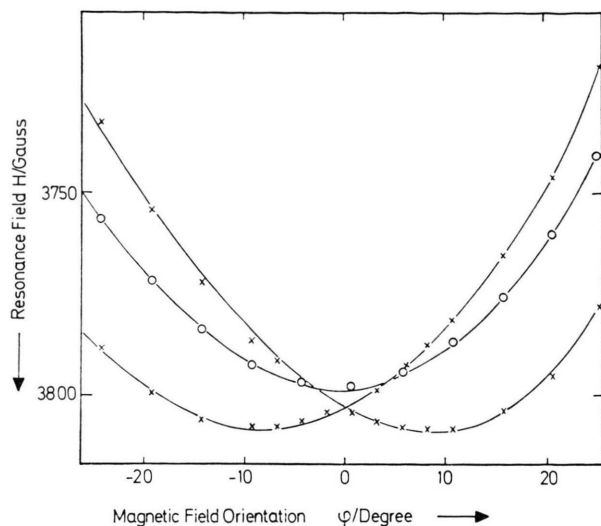
Fig. 3. Fine structure of Anth 0.75 Phen 0.25 -TCNB. Only a small section near H \parallel x ( \phi = 0 ) is shown. The magnetic field is rotated in the molecular xy -plane. "x": T = 102 K, "o": T = 295 K. Microwave frequency: 9336 \pm 2 MHz.
